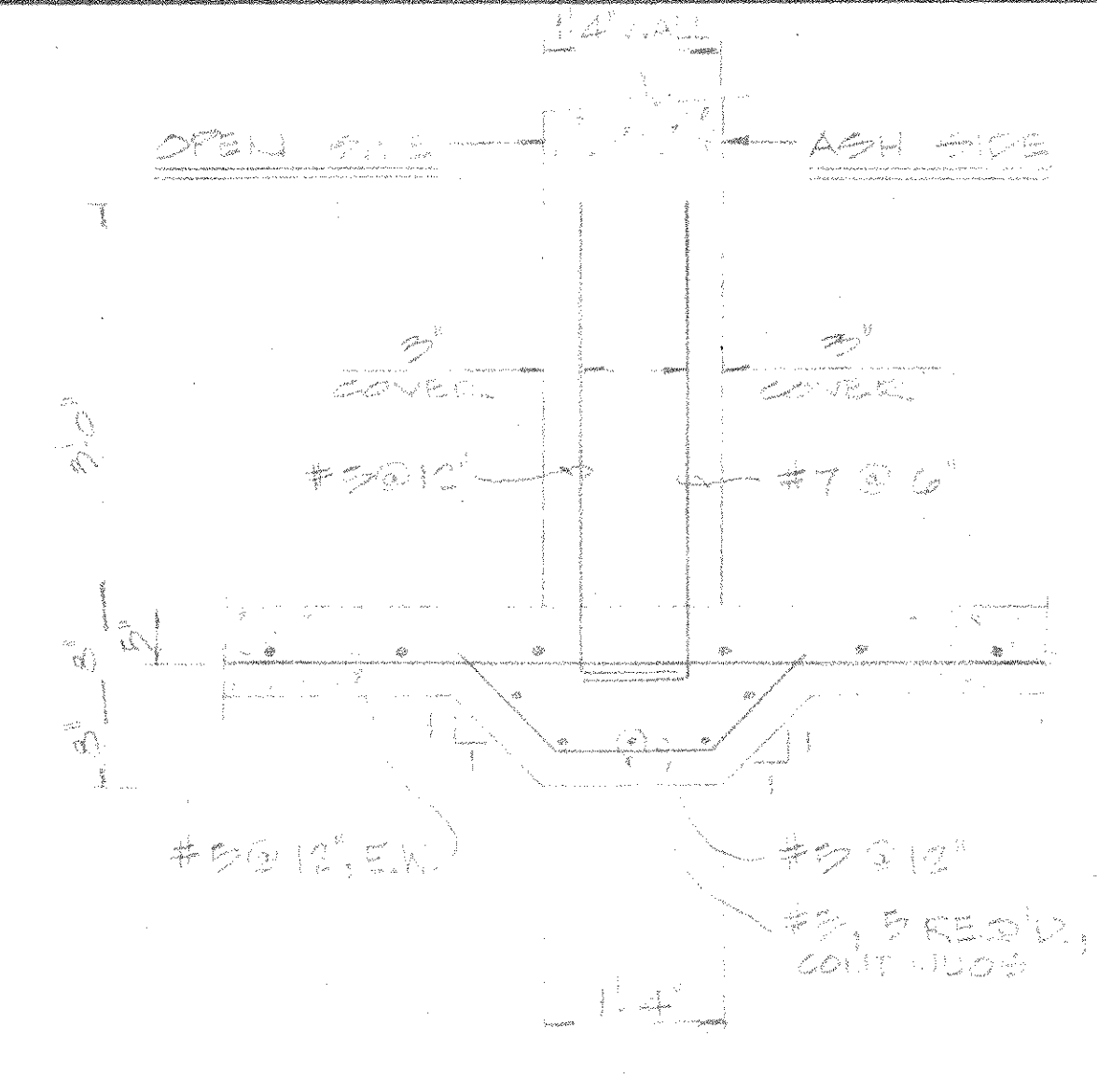
SECTION "C-C"
