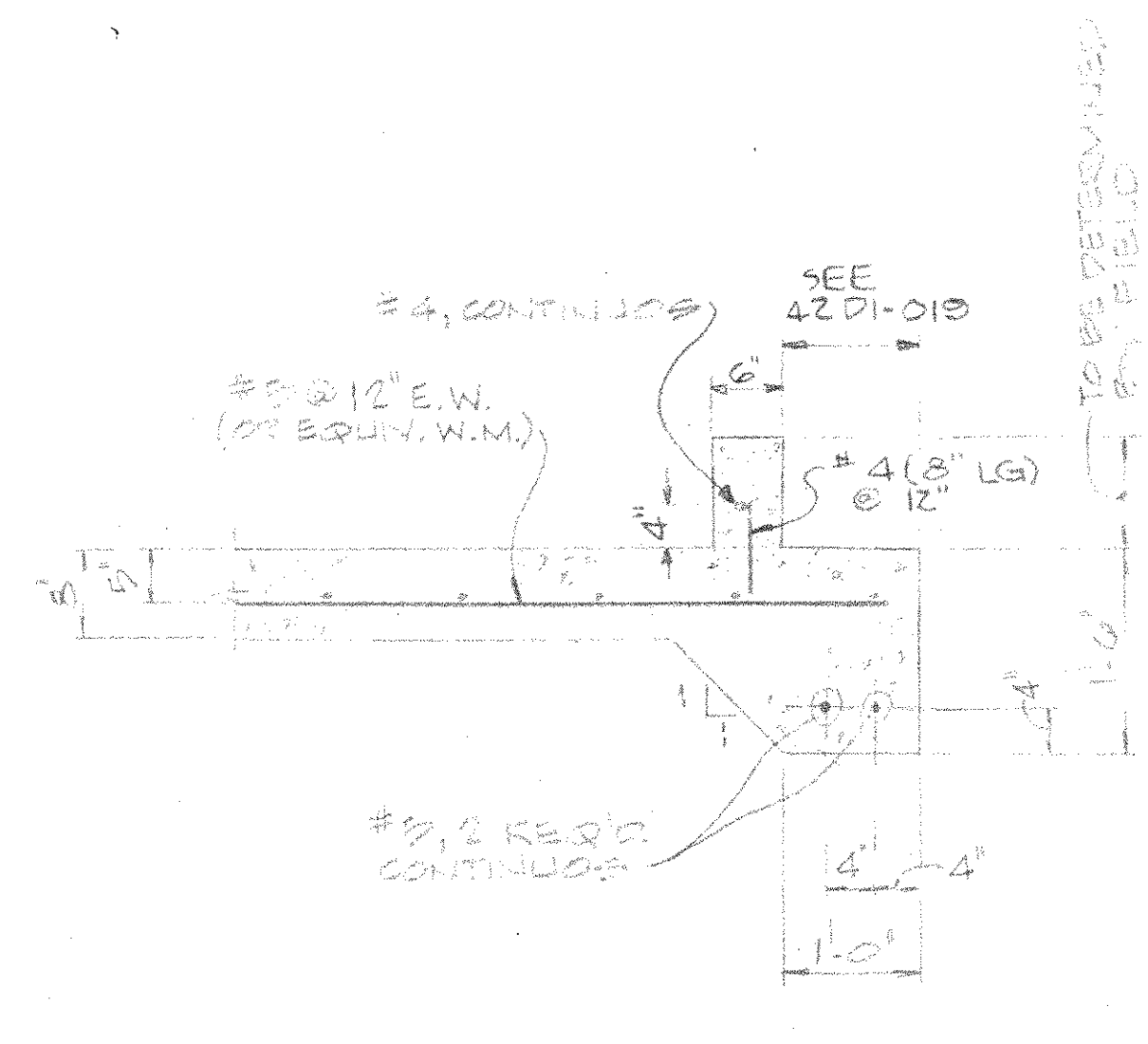
SECTION "B-B"
