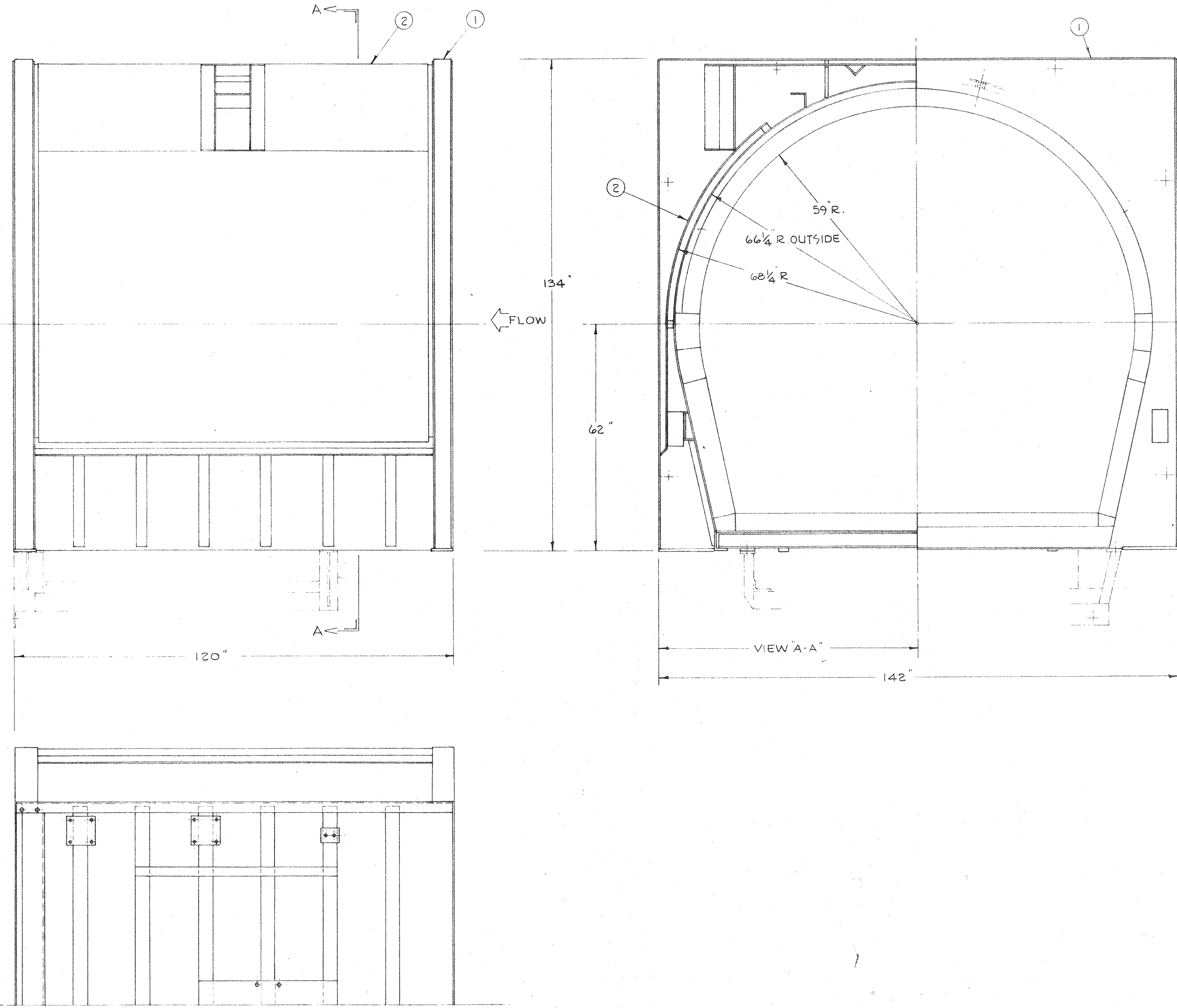
PARTIAL BOTTOM VIEW
