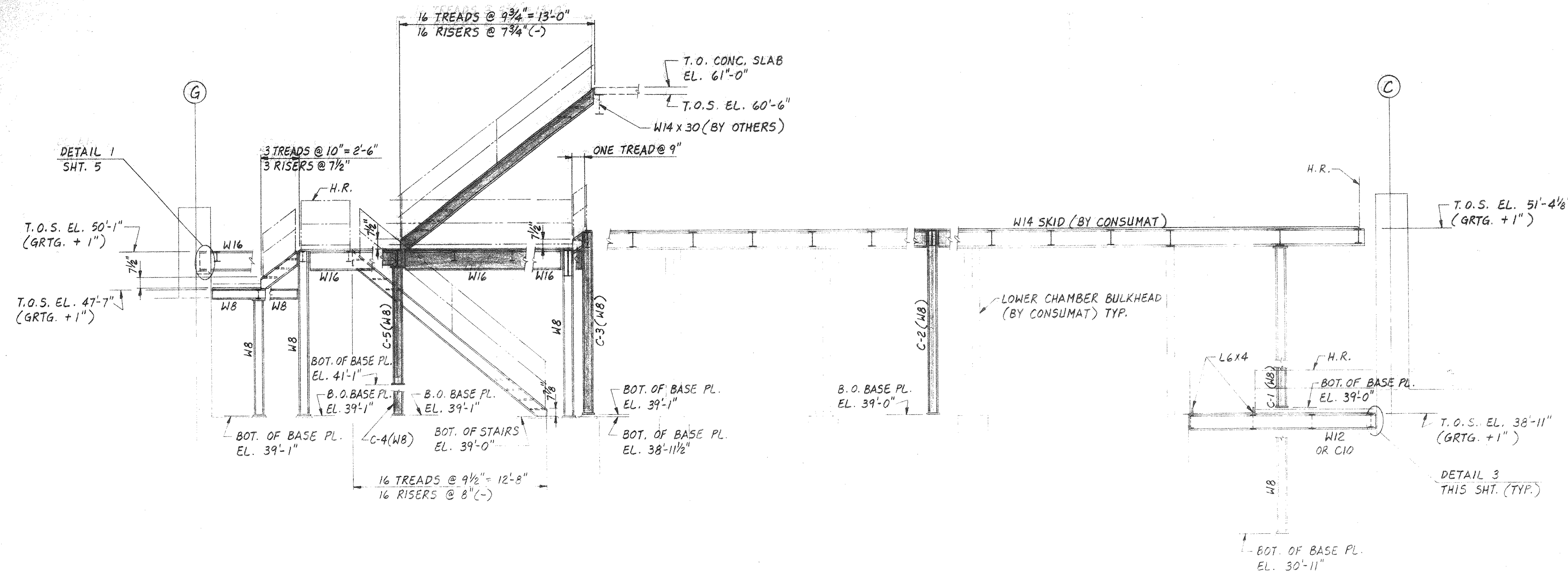
SECTION B-E ELEVATION C-C SCALE: 1/4" = 1'-0"
